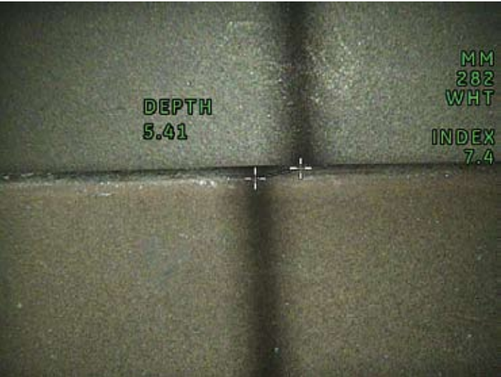
ShadowProbe measurement
