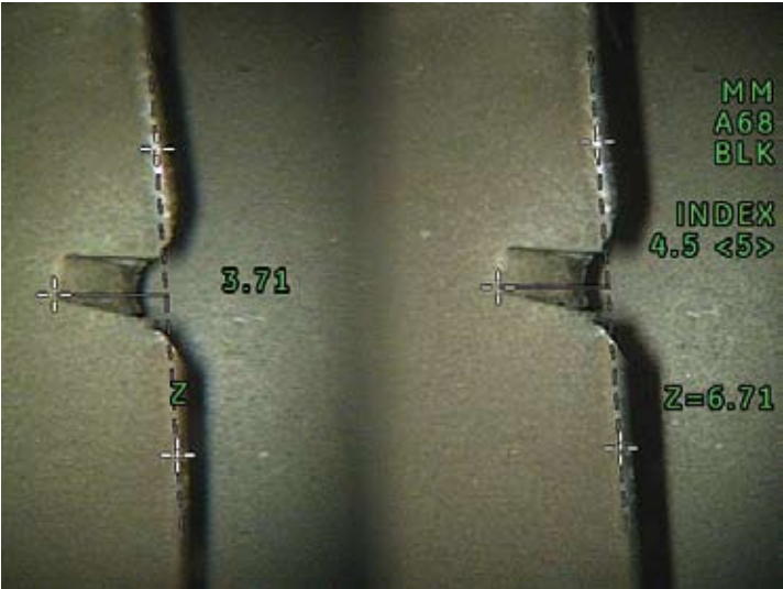
StereoProbe measurement
